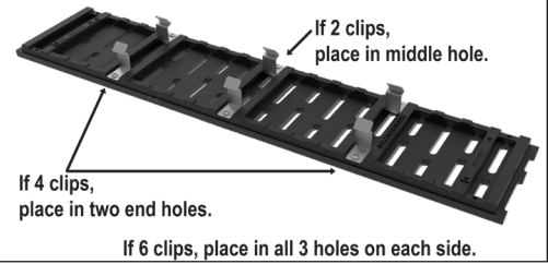
Diagram 1: ClipLock Placement
