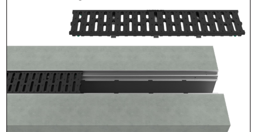
Diagram 4: Grate Installation
