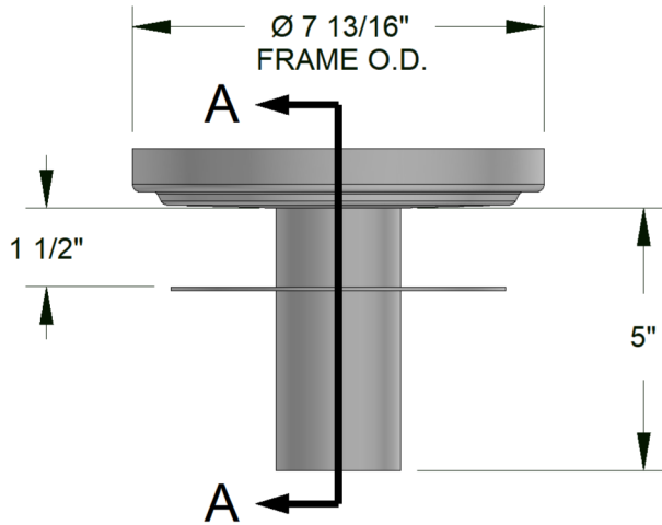
MD FLOOR DRAIN ASSEMBLY SIDE VIEW
