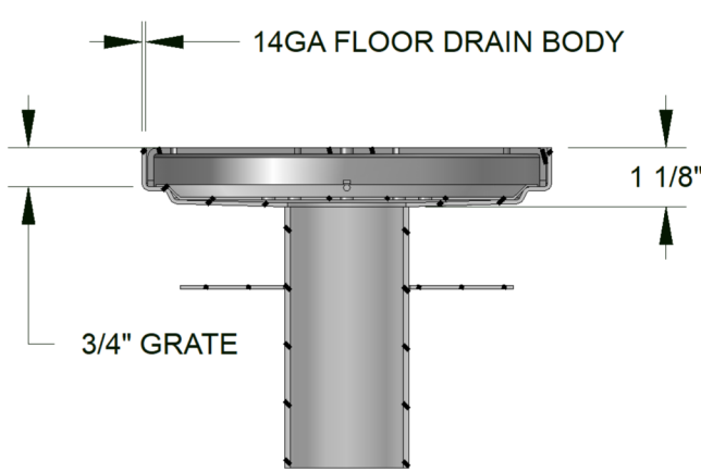
MD FLOOR DRAIN ASSEMBLY SECTION A-A
