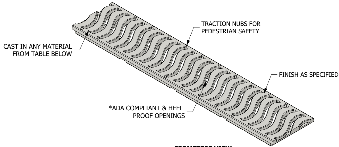
ISOMETRIC VIEW
