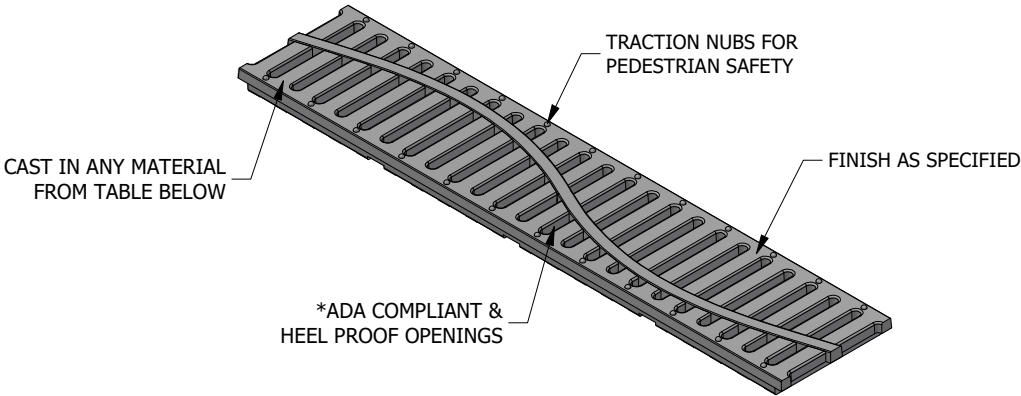
ISOMETRIC VIEW
