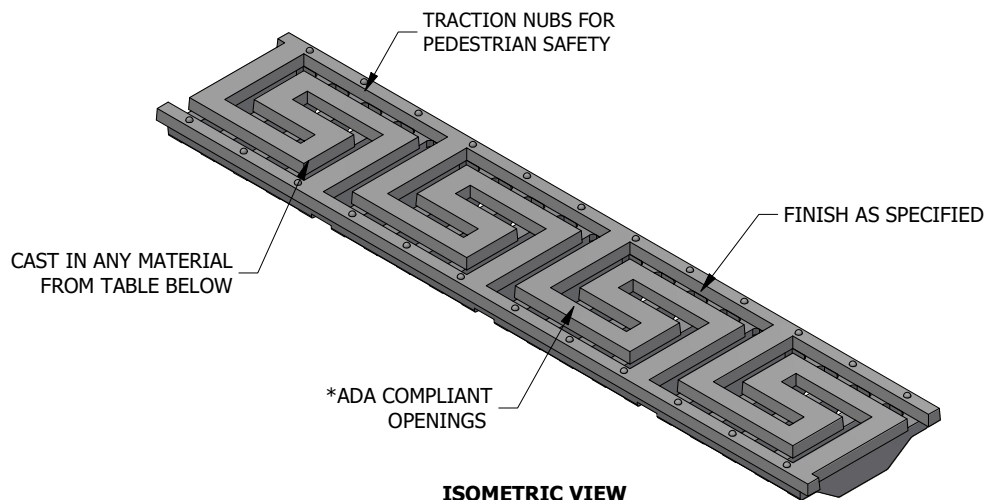
ISOMETRIC VIEW
