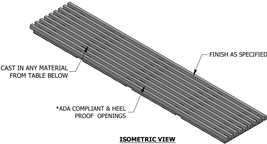
ISOMETRIC VIEW
