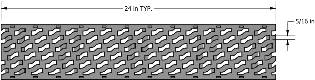
TOP VIEW
