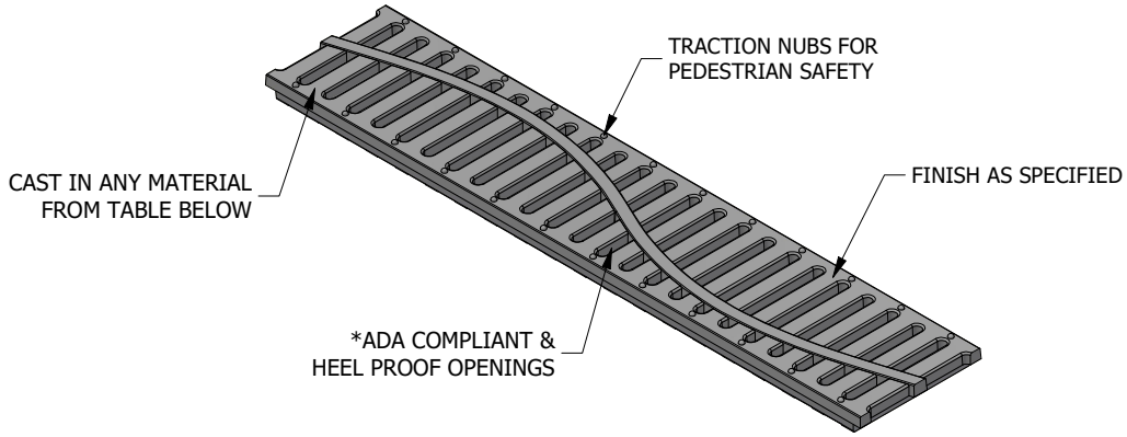
ISOMETRIC VIEW
