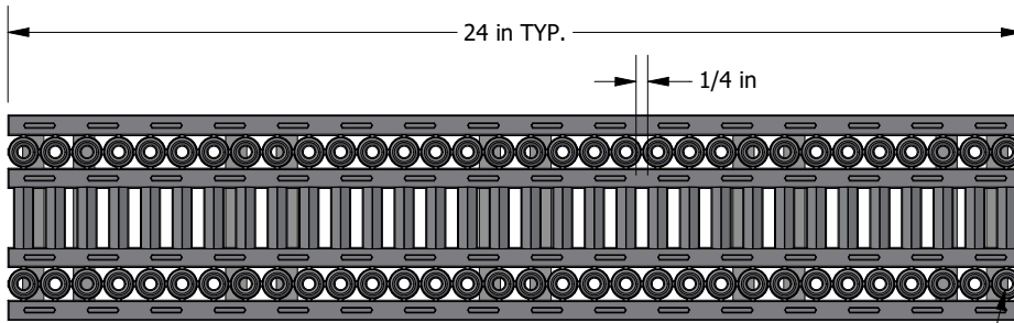
TOP VIEW
