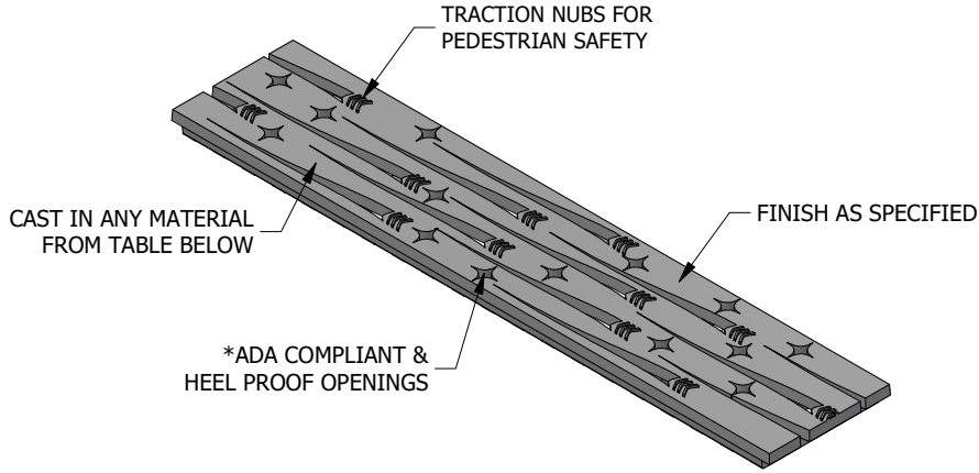
ISOMETRIC VIEW
