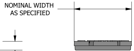
END VIEW
