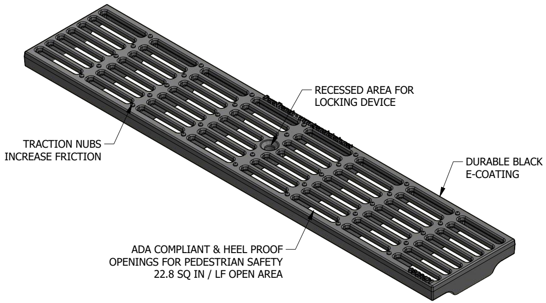
ISOMETRIC VIEW
