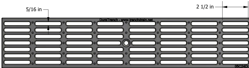
TOP VIEW
