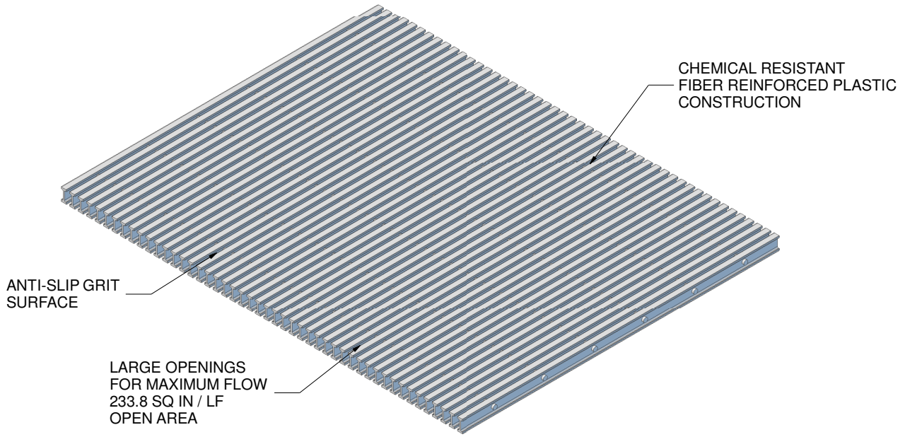
ISOMETRIC VIEW
