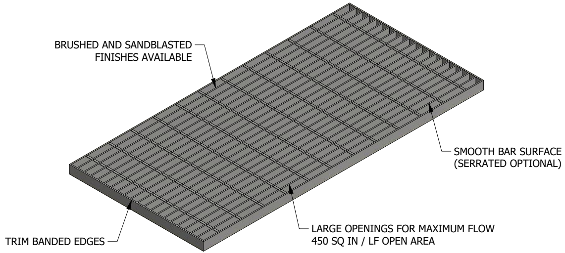
ISOMETRIC VIEW
