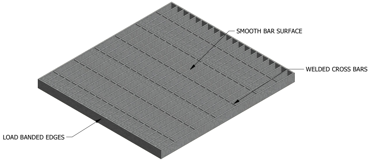
ISOMETRIC VIEW
