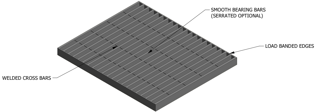
ISOMETRIC VIEW
