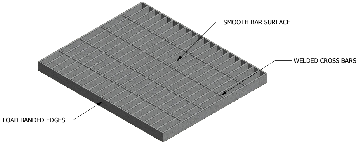
ISOMETRIC VIEW
