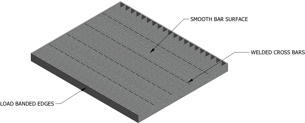
ISOMETRIC VIEW
