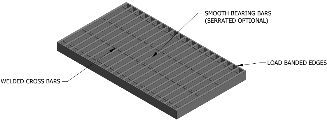
ISOMETRIC VIEW
