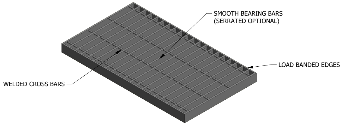
ISOMETRIC VIEW
