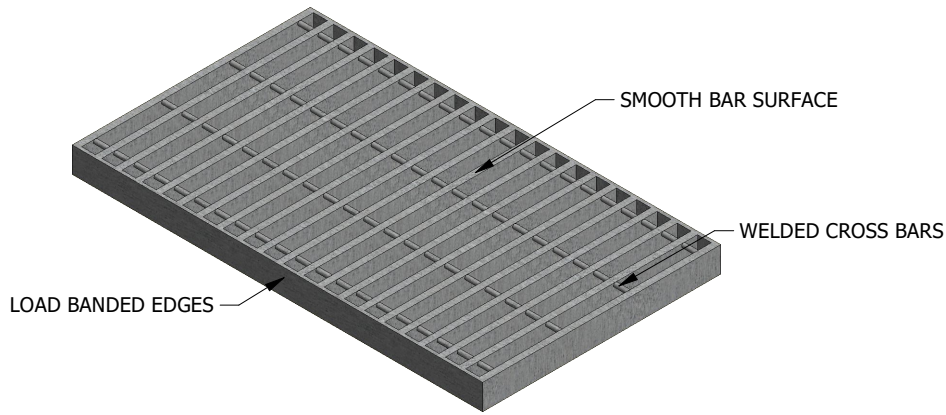
ISOMETRIC VIEW
