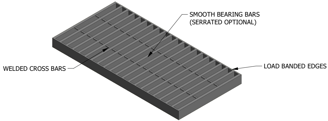
ISOMETRIC VIEW
