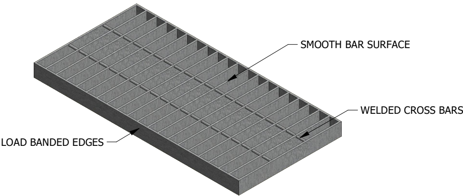
ISOMETRIC VIEW
