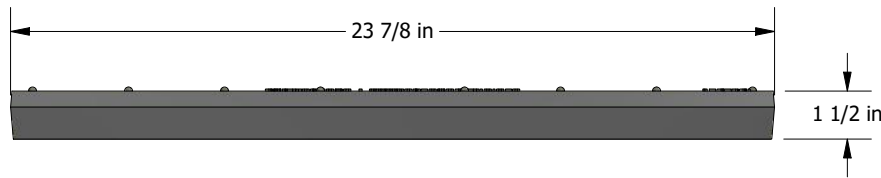
SIDE VIEW
