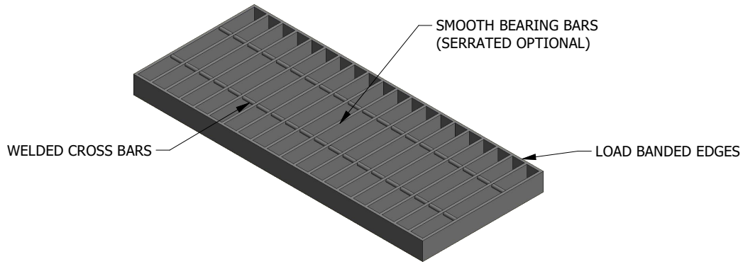
ISOMETRIC VIEW
