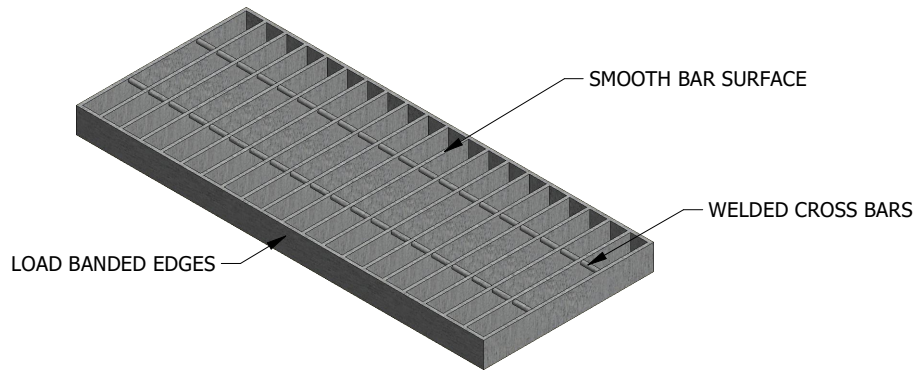
ISOMETRIC VIEW
