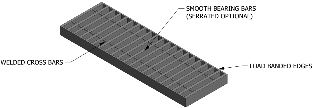
ISOMETRIC VIEW
